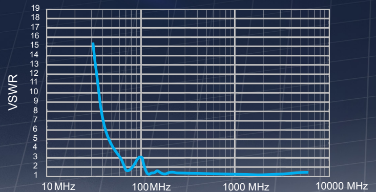
BL-01 - VSWR
